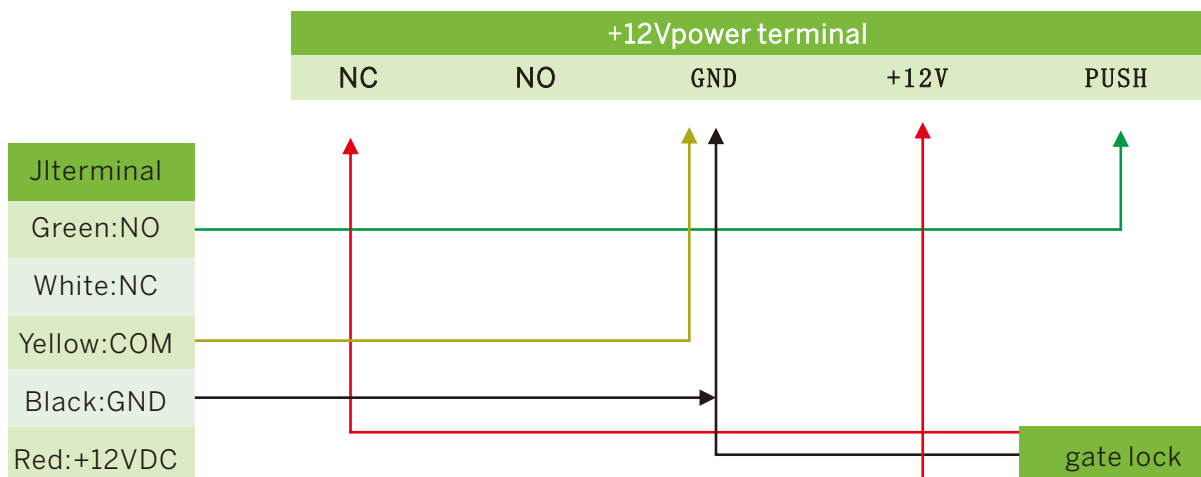
Fig. 1/ 2 schematic diagram of EB-16-R and EB-17-R access control machine wiring
